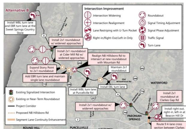
2040 Alternative B: Intersection Capacity Improvements w/ Lane Continuity Enhancement East of Clarks Gap Rd & NB Hillsboro Rd Realignment DRAFT Loudoun County vhb
