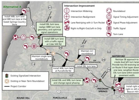
2040 Alternative A: Minor Intersection Improvements Only DRAFT Loudoun County vhb
